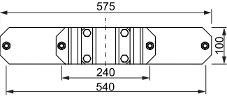
Angle adaptor short WH 01
