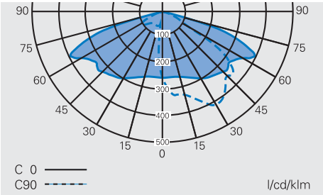
Polar curve PXLED 5L - 30L, asymmetric 2
