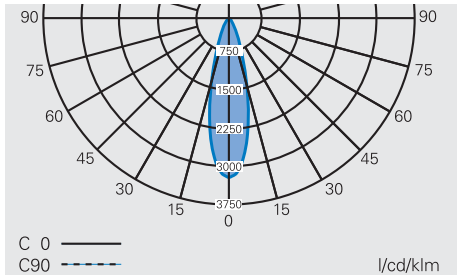
Polar curve PXLED 5L - 30L, asymmetric 1
