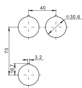
Mounting pitches
