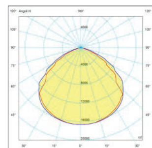
SLED-1001 Luminous flux: 58045 lm
