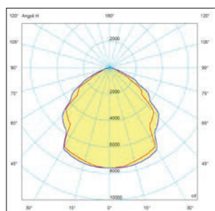
SLED-401 Luminous flux: 18490 lm
