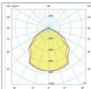
SLED-250 Luminous flux: 12387 lm
