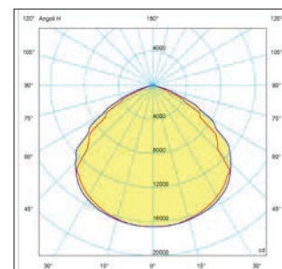
SLED-600 Luminous flux: 30799 lm
